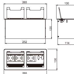
Outline Drawing:
