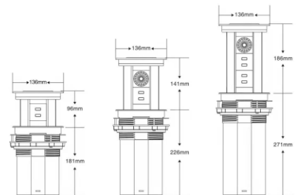
Outline Drawing:
