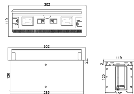
Outline Drawing:
