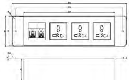
Outline Drawing:
