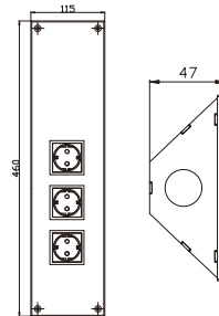
Outline Drawing:
