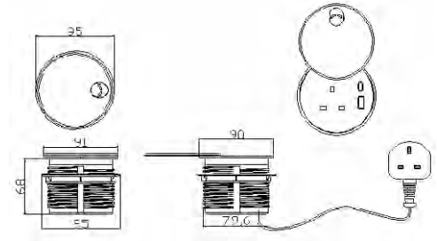
Outline Drawing:
