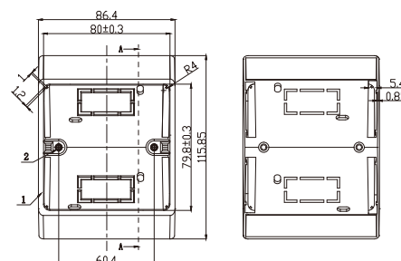
Outline Drawing:
