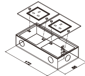
Outline Drawing:
