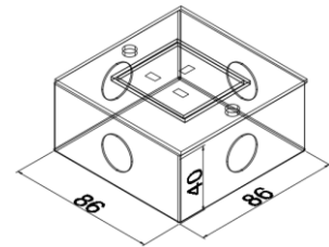
Outline Drawing:
