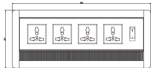
Outline Drawing:
