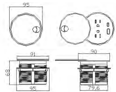
Outline Drawing:
