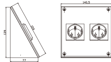
Outline Drawing:
