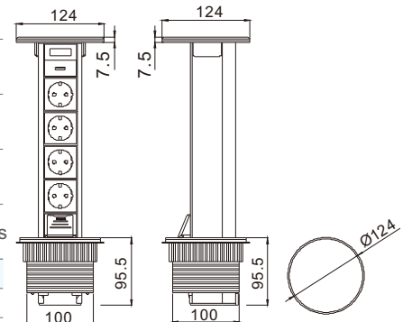
Outline Drawing:
