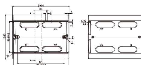
Outline Drawing:
