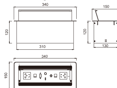
Outline Drawing:
