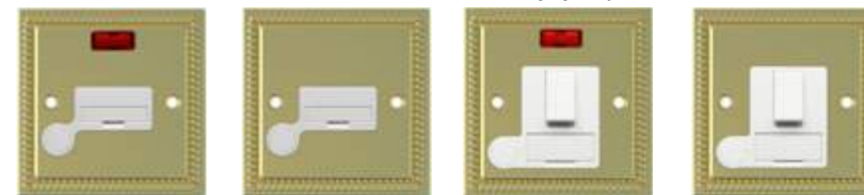
BH413 13A fused connection unit+neon+flex outlet BH414 5A fused connection unit+neon+flex outlet BH415 3A fused connection unit+neon+flex outlet BH416 13A fused connection unit+flex outlet BH417 5A fused connection unit+flex outlet BH418 3A fused connection unit+flex outlet BH419 13A switched FCU'S+neon+flex outlet BH420 5A switched FCU'S+neon+flex outlet BH421 3A switched FCU'S+neon+flex outlet BH422 13A switched FCU'S+flex outlet BH423 5A switched FCU'S+flex outlet BH424 3A switched FCU'S+flex outlet
