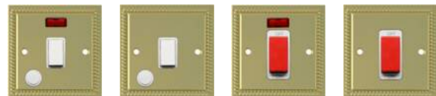
BH3240 20A 1 gang double pole switch + neon+flex outlet BH3250 20A 1 gang double pole switch+flex outlet BH327 45A 1gang double pole switch+neon, single plate BH328 45A 1 gang double pole switch, single plate
