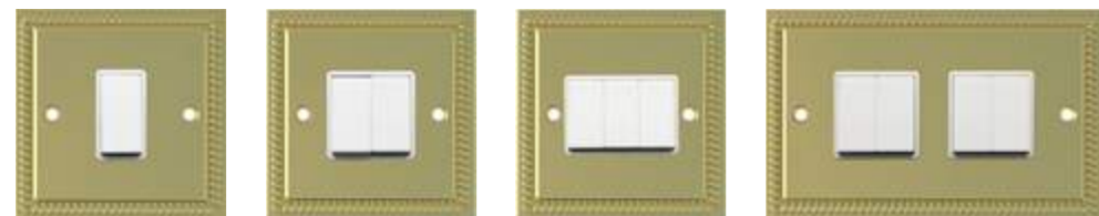
BH301 1 gang 1 way plate switch BH302 1 gang 2 way plate switch BH303 2 gang 1 way plate switch BH304 2 gang 2 way plate switch BH305 3 gang 1 way plate switch BH306 3 gang 2 way plate switch BH307 4 gang 1 way plate switch BH308 4 gang 2 way plate switch
