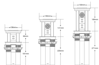
Outline Drawing:
