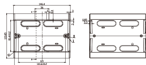
Outline Drawing:
