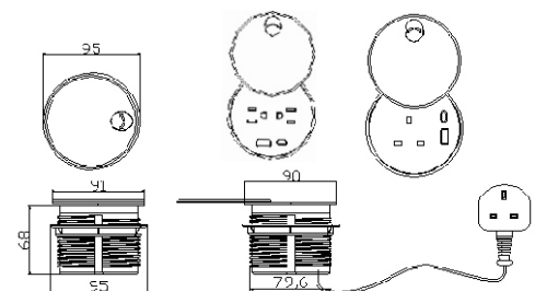
Outline Drawing:
