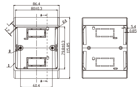
Outline Drawing:
