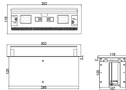
Outline Drawing:
