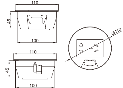
Outline Drawing:
