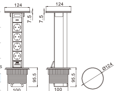
Outline Drawing:
