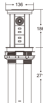
Outline Drawing:
