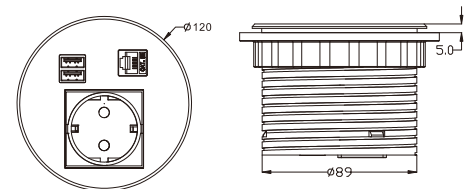
Outline Drawing:
