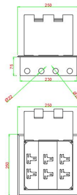
HTD-250K-86 outline
