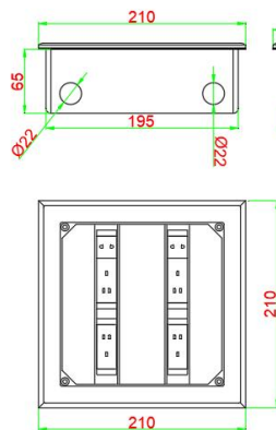
HTD-210CK
