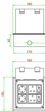
HTD-180K outline
