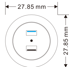
Outline Drawing:
