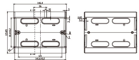
Outline Drawing:
