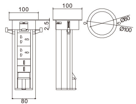
Outline Drawing:
