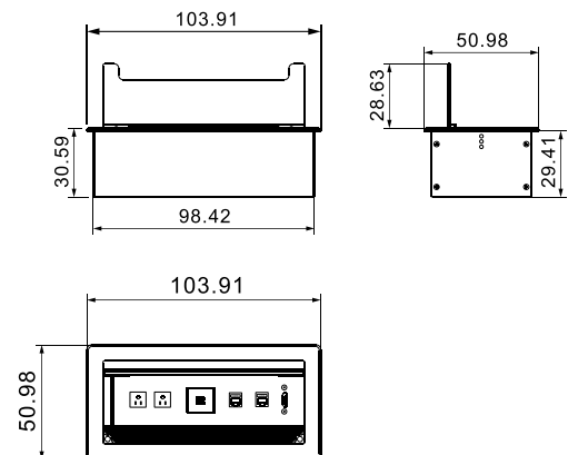
Outline Drawing:
