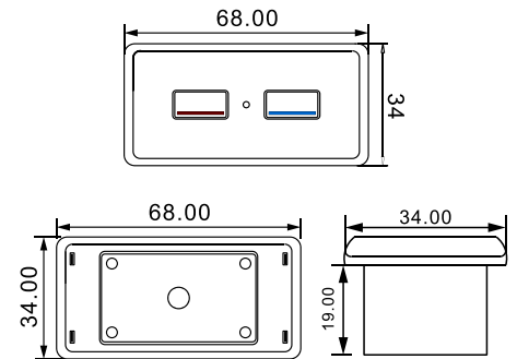
Outline Drawing:
