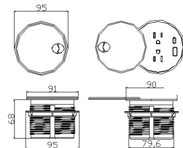
Outline Drawing:
