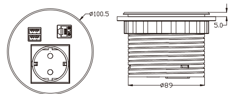
Outline Drawing:
