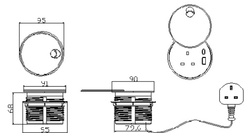
Outline Drawing:
