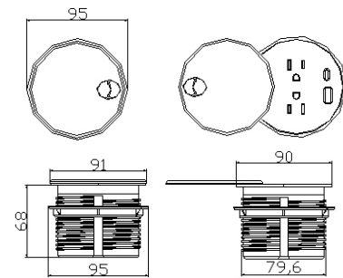
Outline Drawing:
