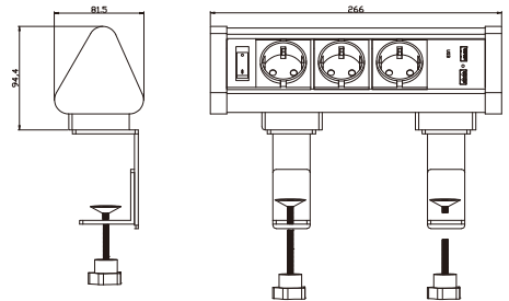
Outline Drawing:
