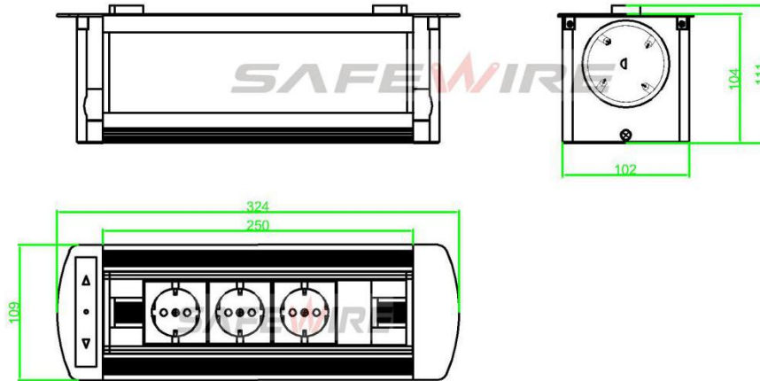
FZ-561E outline
